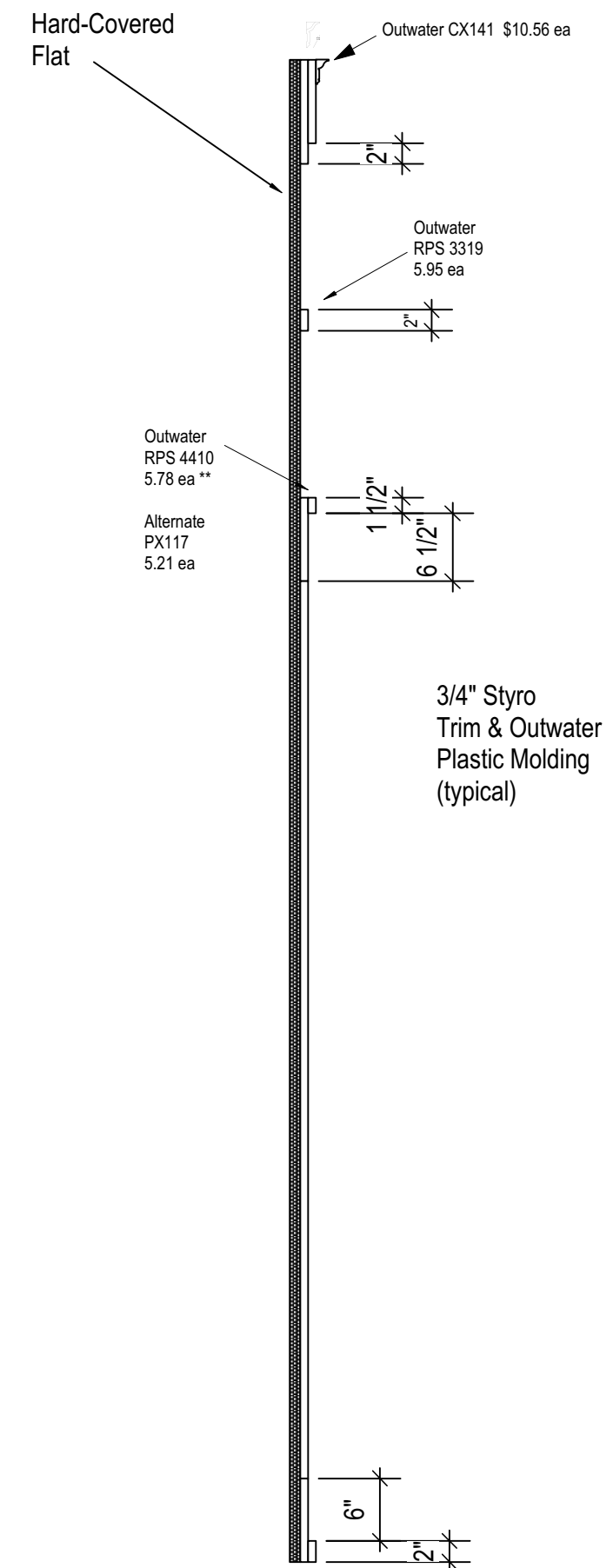
Trim Detail- Section View (Typical)
